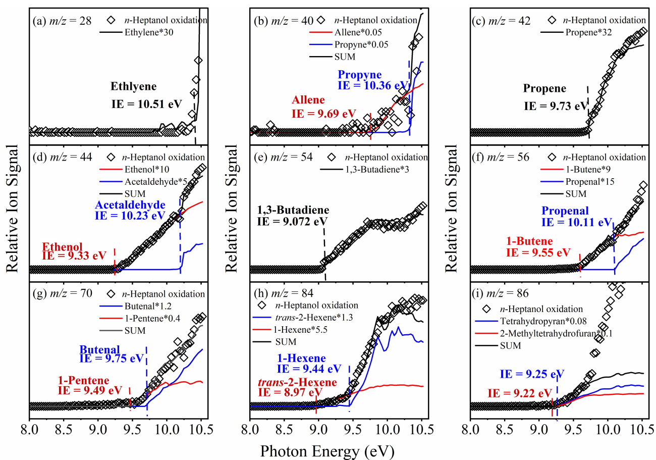
Fig. S1 The PIE spectra of main oxidation products of n -heptanol detected in this work.
