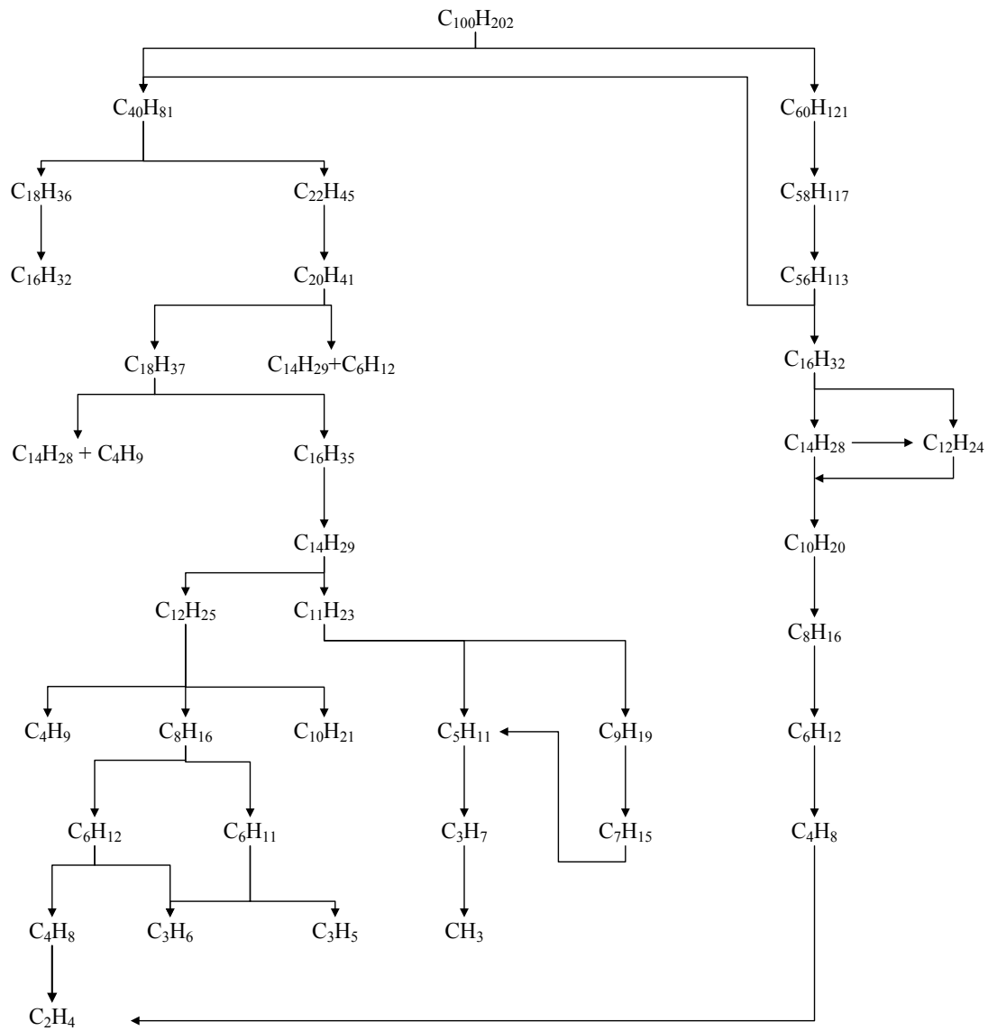
Fig. 1 Typical path of PE pyrolysis to C_2H_4
