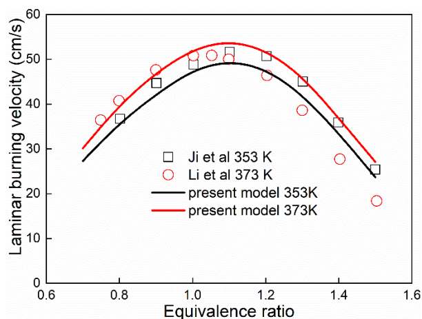
Figure S3 Comparison of the measured laminar burning velocities of n -hexane/air at 353 K, 1 atm by Ji et al. [7] and 373K, 1 atm by Li et al. [8] (symbols) and simulated results of the present model (lines).
