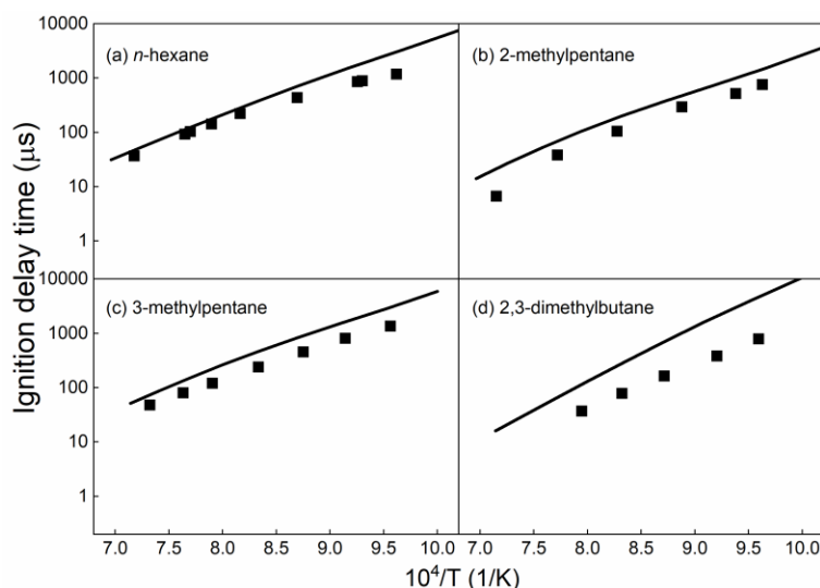
Figure S2 Comparison of the measured ignition delay times of (a) n -hexane (b) 2-methylpentane (c) 3-methylpentane (d) 2,3-dimethylbutane at 15 atm by Zhang et al. [6] (symbols) and simulated results of the present model (lines).
