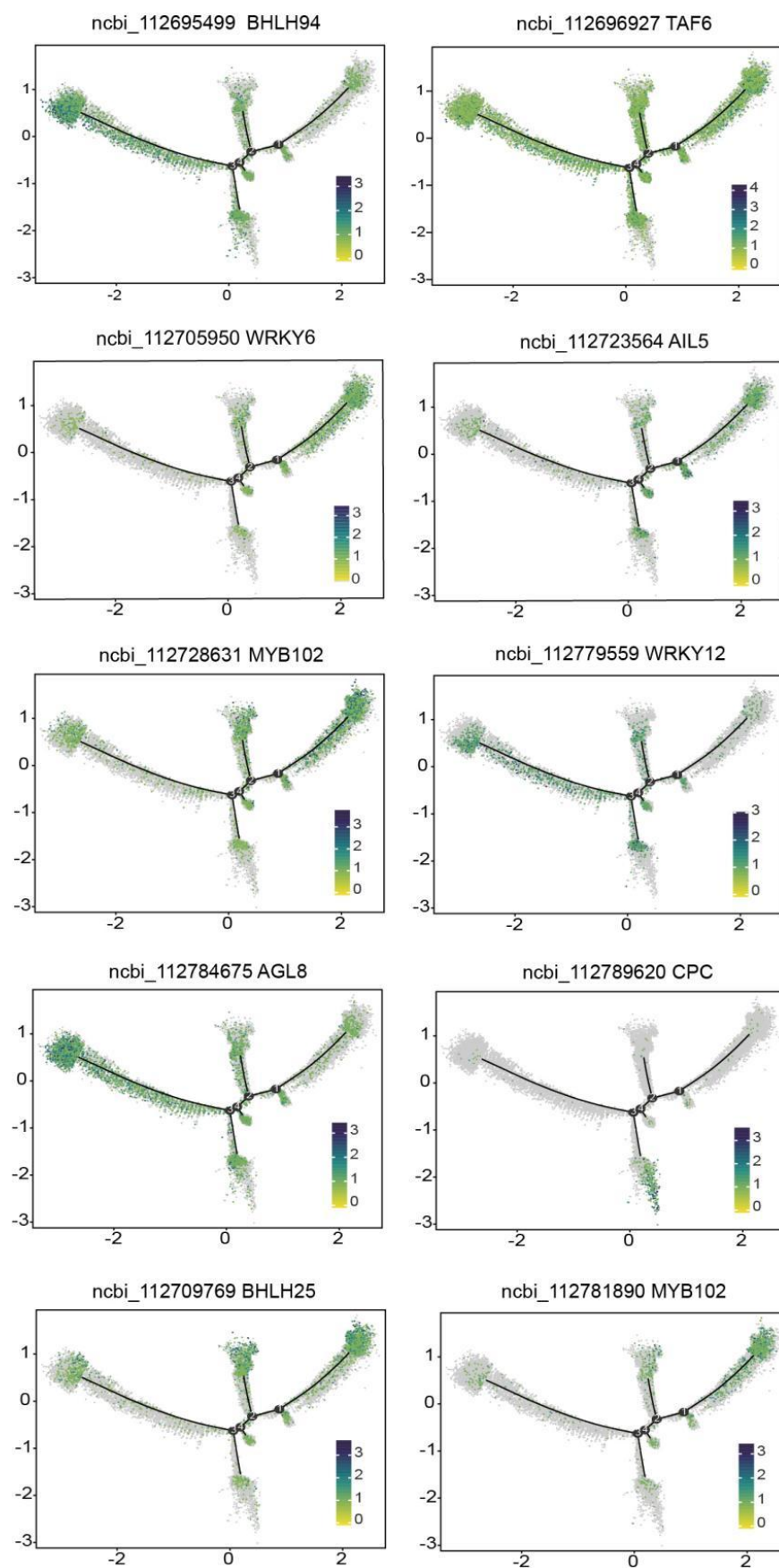
Fig. S10 The expression patterns of ten TFs along the subterranean peg cell differentiation trajectory
