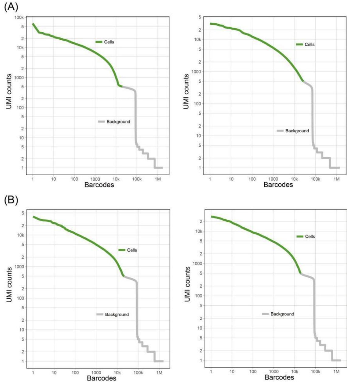
Fig. S1 Knee plots and empty drop cutoffs identified by the Cell Ranger filtering algorithms in aerial and subterranean pegs. A Two replicates in aerial pegs; B Two replicates in subterranean pegs
