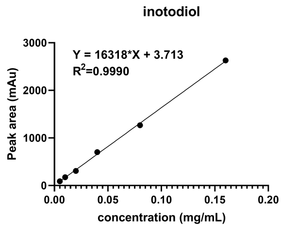
Supplementary Figure S3. Calibration curve for inotodiol quantification.
