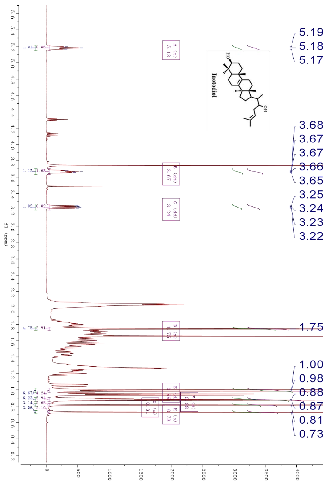
Supplementary Figure S1. ^1\text{H} nuclear magnetic resonance ( ^1\text{H} -NMR) spectrum of inotodiol (measured in \text{CDCl}_3 at 500 MHz).
