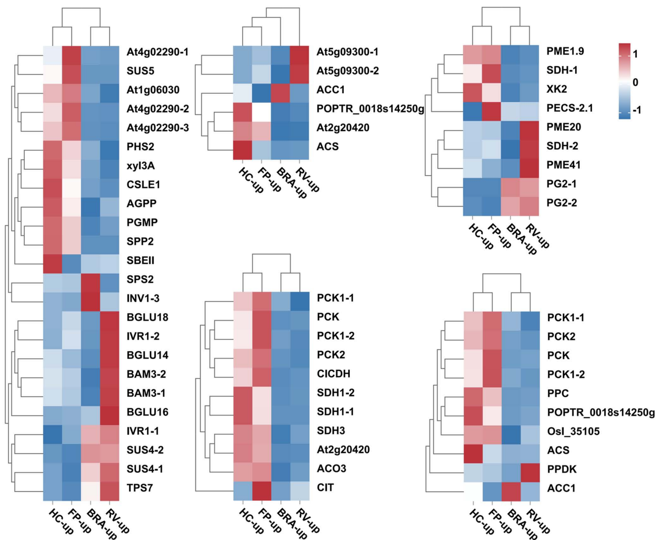
Fig. S4. Heatmap analysis of differentially expressed genes (DEGs) in carbohydrate metabolism. A: Starch and sucrose metabolism; B: propanoate metabolism; C: citrate cycle (TCA cycle); D: pentose and glucuronate interconversions; E: pyruvate metabolism. Colored scale top indicates the FPKM value.
