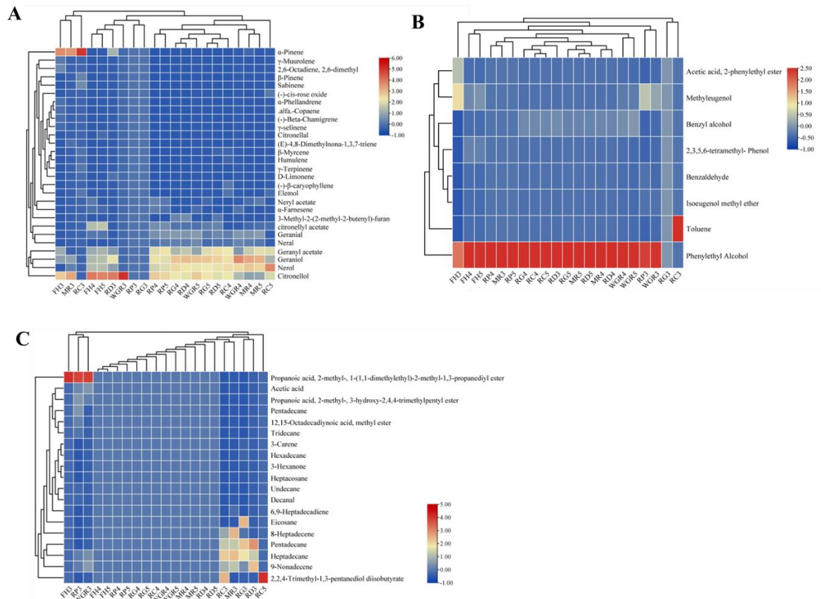
Figure S1. Heatmap Cluster Analysis of different biosynthesis pathway.
