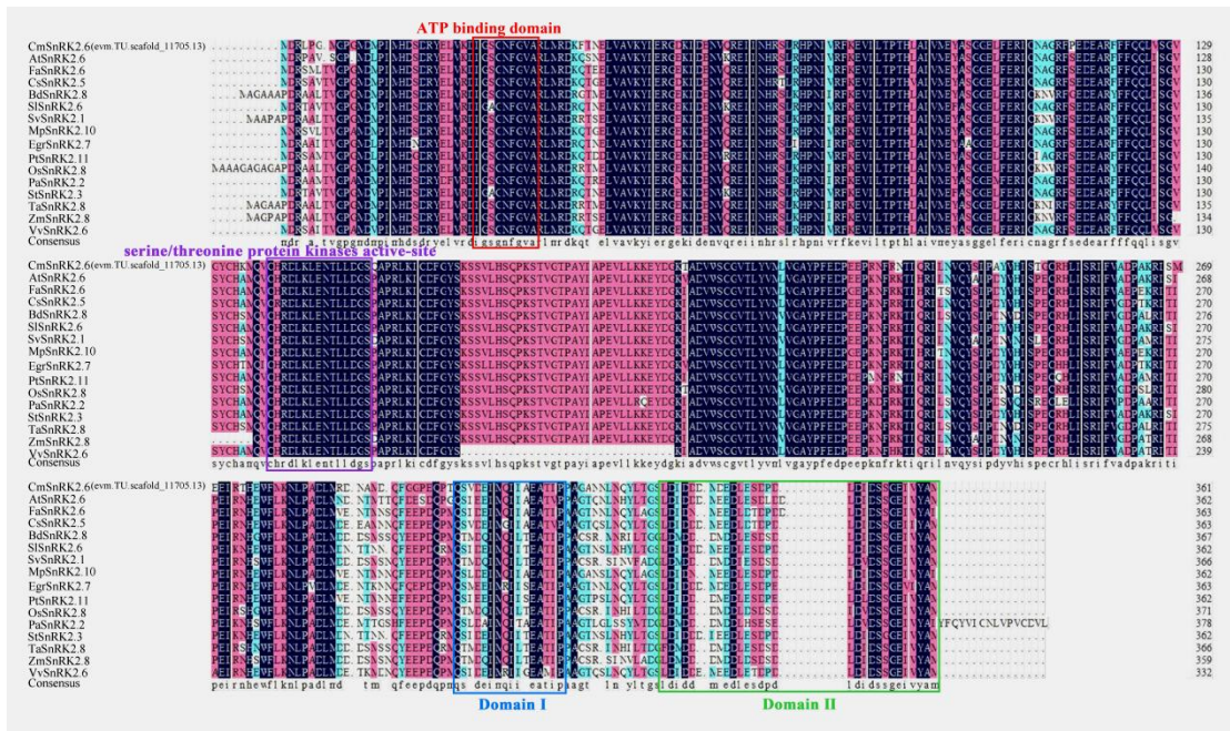
Supplementary Fig. S10 Analysis of amino acid sequences of 16 SnRK2 proteins.
