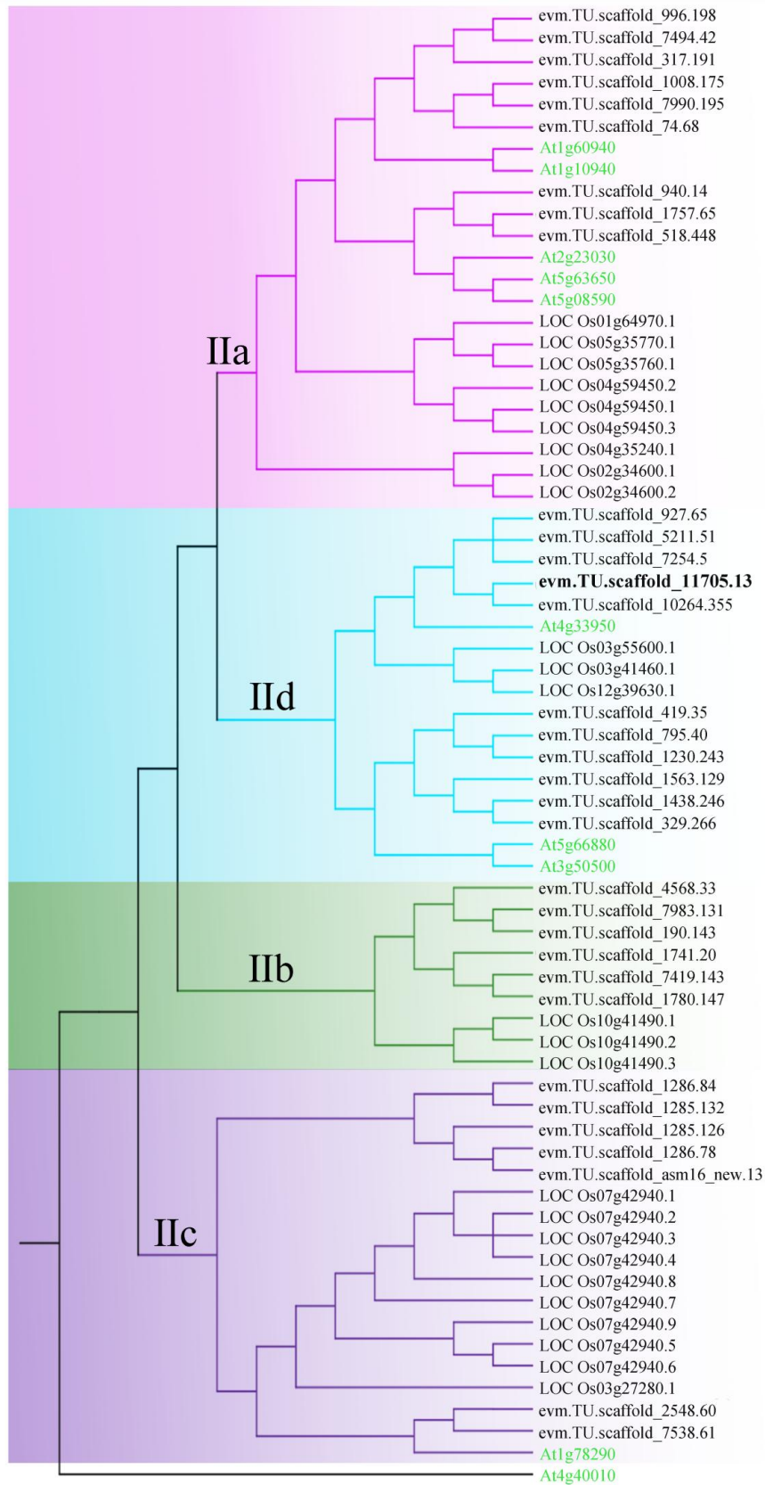
Supplementary Fig. S9 Phylogenetic tree of SnRK2 proteins from the 'f23' transcriptome, Arabidopsis, and rice based on kinase domain amino acid sequences (Poisson correction model).
