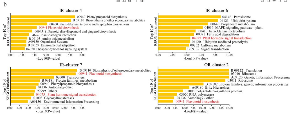
Supplementary Fig. S5 Co-expression clustering analysis of inner and outer ray florets during the post-flowering stage in 't23'. (a) Gene expression heatmap of inner and outer ray florets during the post-flowering stage. (b) Focused gene cluster from KEGG enrichment analysis of genes in inner and outer ray florets during the post-flowering stage.
