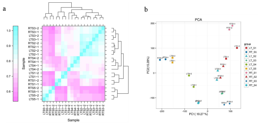
Supplementary Fig. S3 Correlation analysis and principal component analysis (PCA) of all transcripts and expressed genes in D.nobile . (a) Correlation analysis of expressed genes among different samples from different treatments. (b) PCA plot of all transcriptome results.
