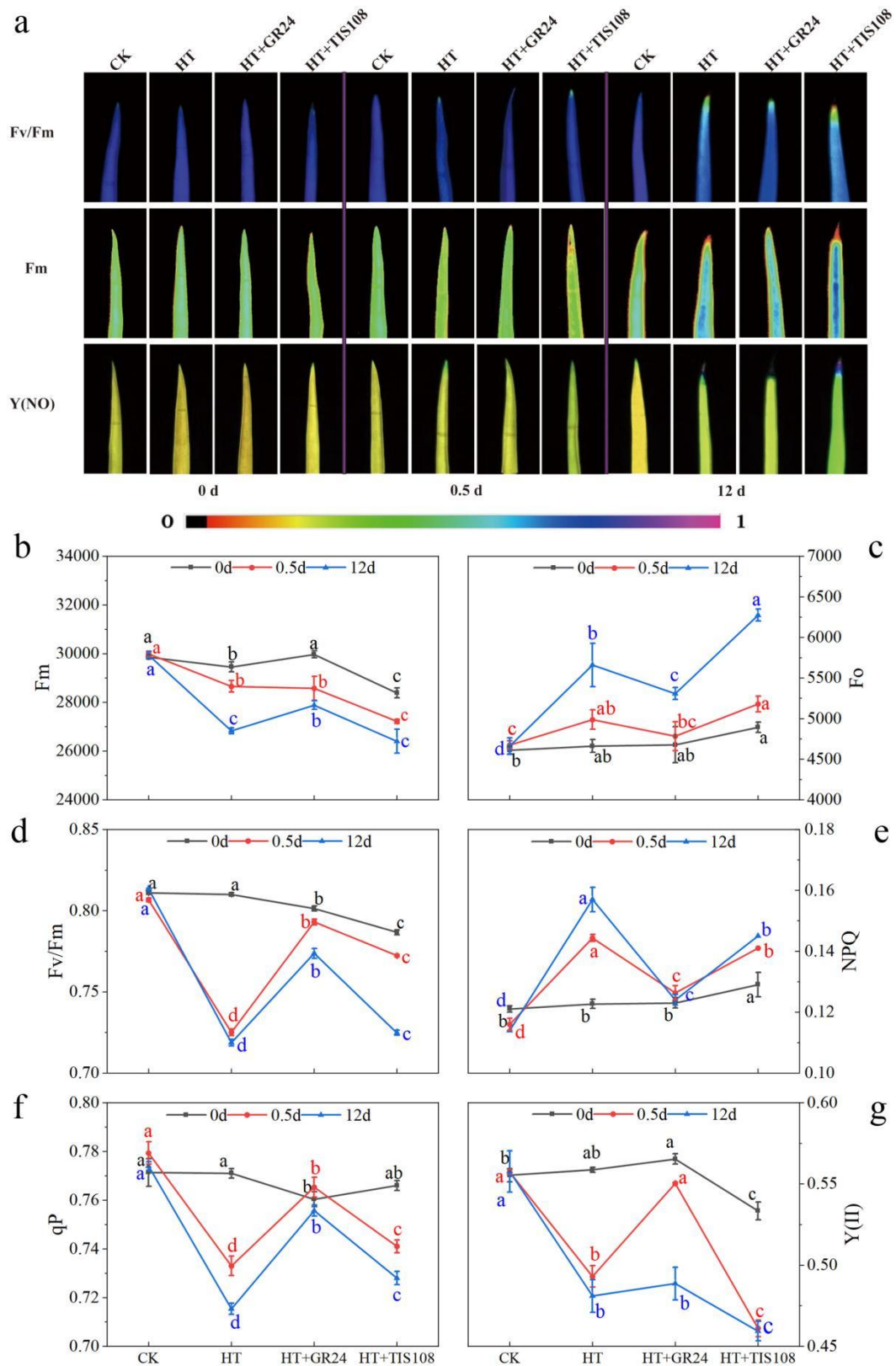
Fig. S2 Effects of pre-spraying with GR24 and TIS108 on chlorophyll fluorescence parameters of carnation seedlings under HS. (a) Chlorophyll fluorescence phenotype. (b) F_m . (c) F_o . (d) F_v/F_m . (e) NPQ. (f) qP . (g) Y(II) . Data shown as mean \pm SD, and different letters indicate significant differences ( P < 0.05 ).
