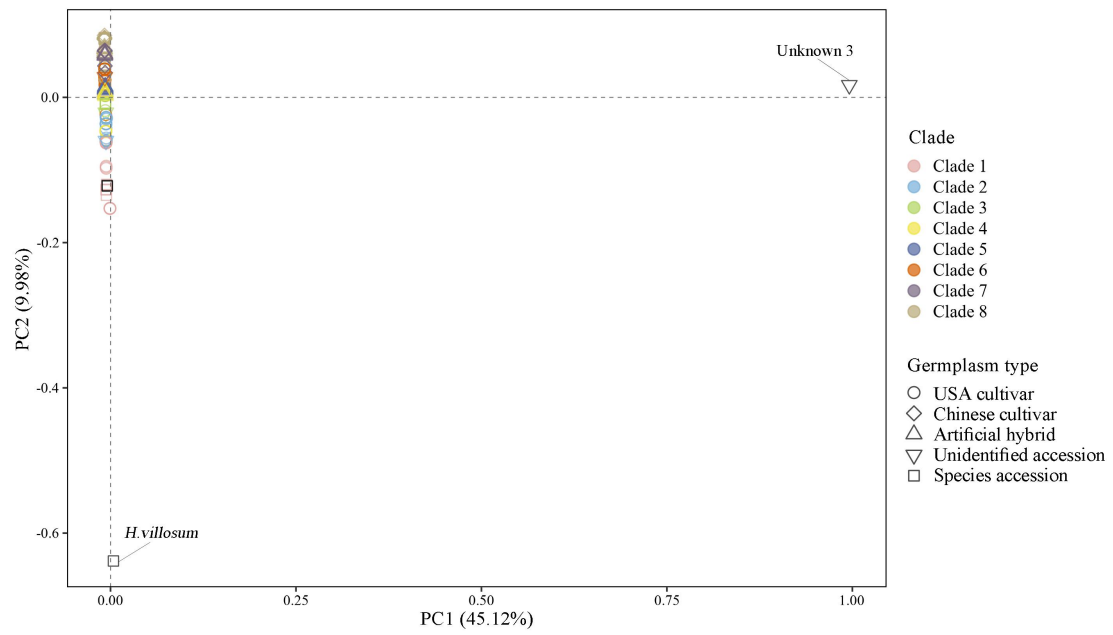
Fig. S1 Preliminary PCA of all 167 Hedychium samples based on 265,365 SNPs after LD pruning. H. villosum and Unknown 3 showed marked divergence from the remaining samples.
