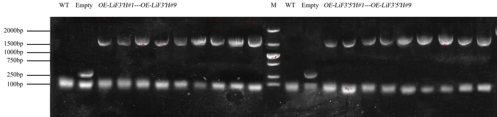
Supplementary Fig.S2 The PCR results of genetically modified tobacco.
