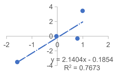
i0_LQ_BZL_c3200/f1p0/940
