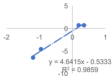
i1_HQ_BZL_c50082/f2p0/1631
