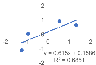
i1_HQ_BZL_c17400/f3p13/1627
