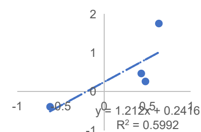
i4_HQ_BZL_c21648/f2p0/4553
