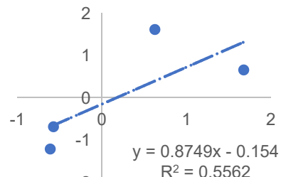
i1_LQ_BZL_c24884/f1p3/1545
