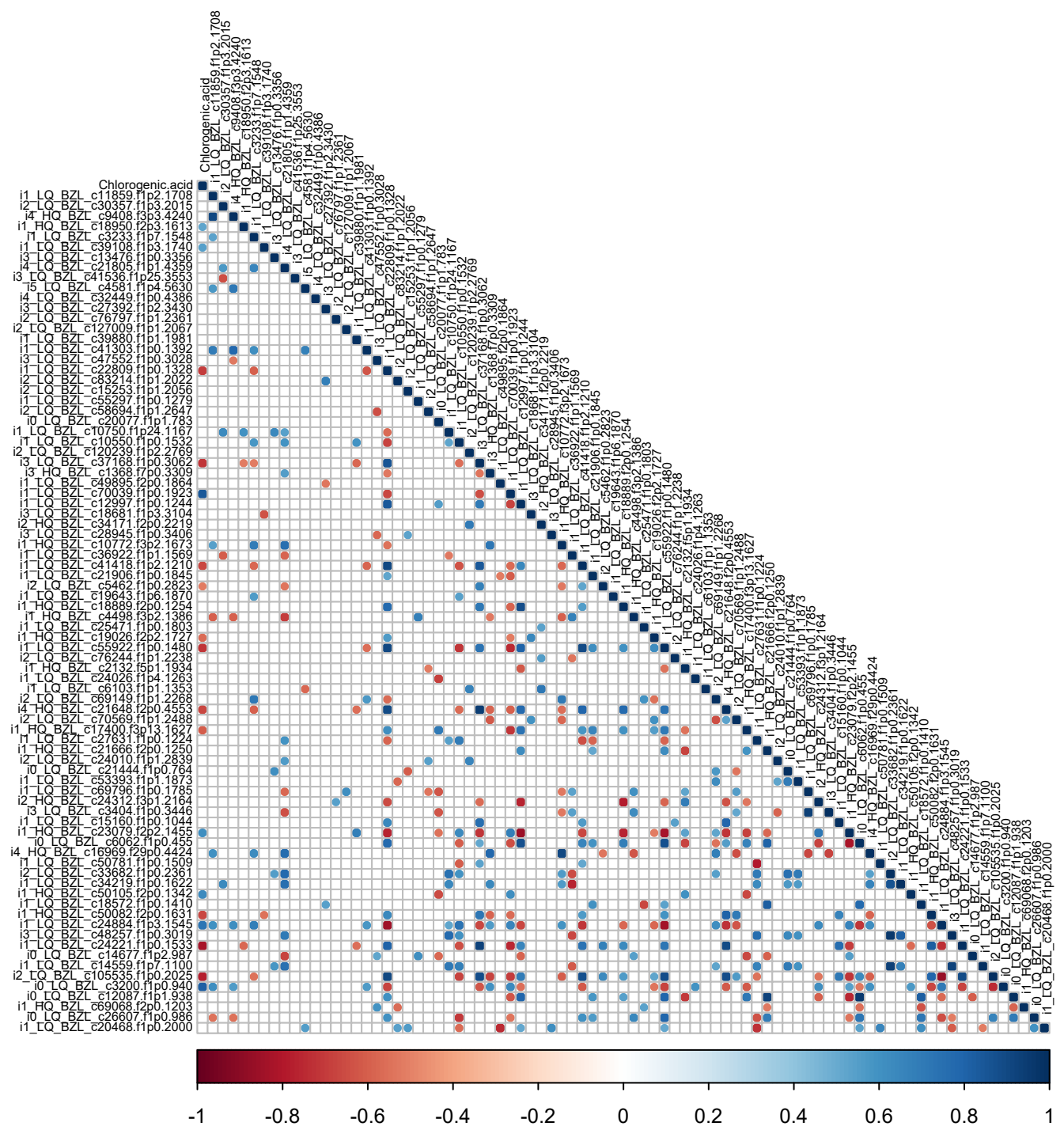
Supplementary Figure 3. The corrplot represents the correlation between CGA content and the expression levels of 75 MYB transcription factor and 8 HQT genes.
