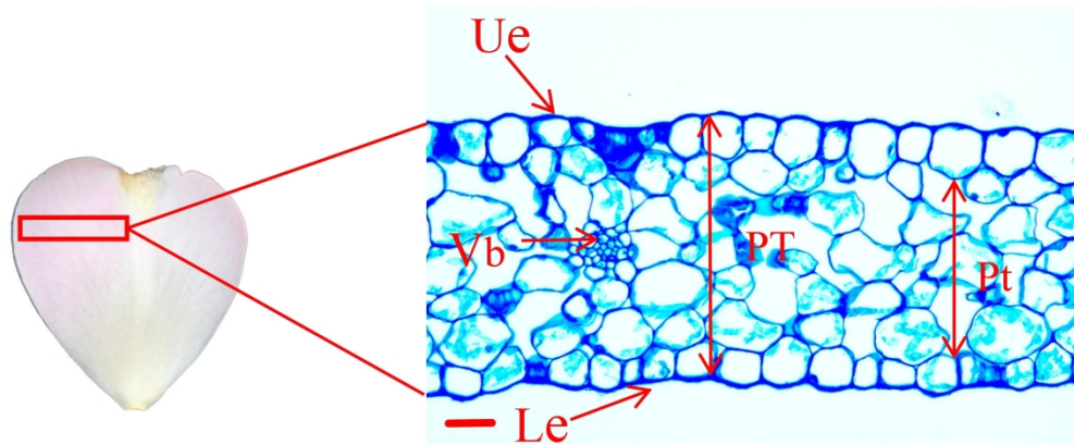
Fig. S2. Petal anatomical structure of 'Tongzimian'. Scale Bar=40 \mu m; Ue: Upper epidermis; Le: Lower epidermis; PT: Petal thickness; Pt: Parenchyma tissue; Vb: Vascular bundle.
