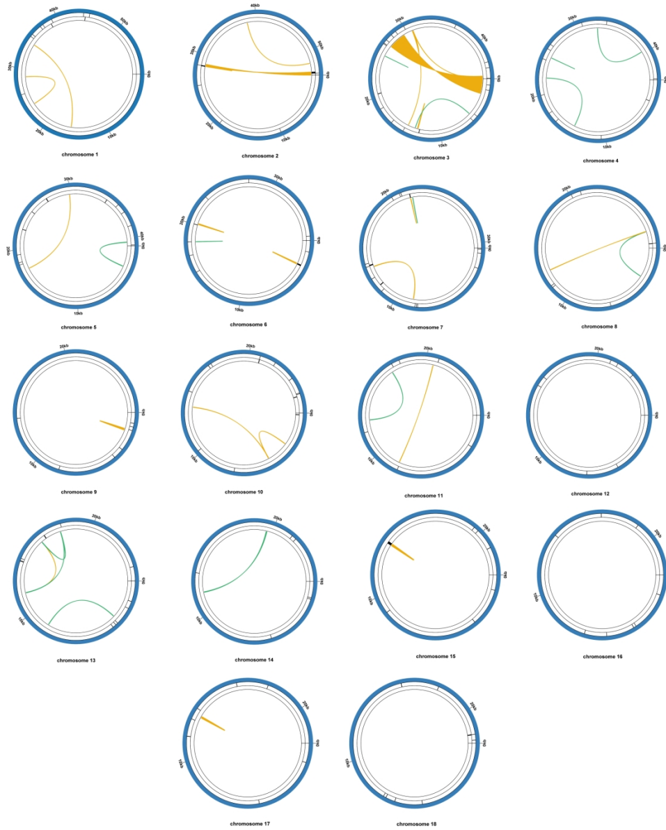
Fig. S2. Chordal diagram of repeated sequences of D. chrysotoxum .
