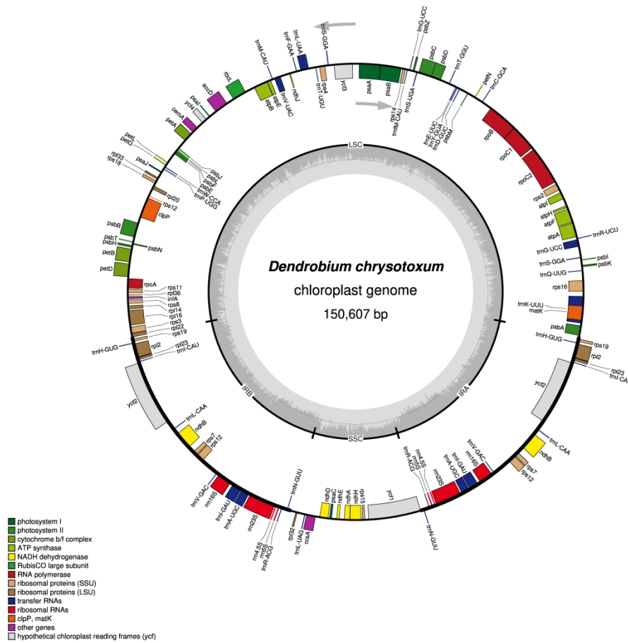
Fig. S1. D. chrysotoxum map of the chloroplast genome.
