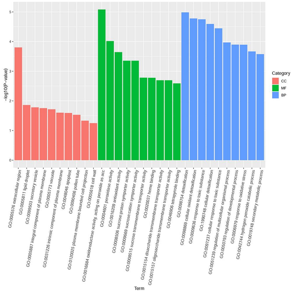
Fig. S2. GO functional classification of DEGs. DEGs were identified in three categories: molecular function (MF, green), cellular component (CC, red) and biological process (BP, blue).
