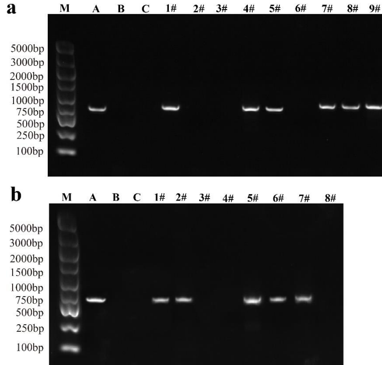
Supplementary Figure S1. PCR identification of Arabidopsis transformed with HmWOX8 gene. (a) PCR identification of HmWOX8 gene overexpression strain; (b) PCR identification of HmWOX8 gene recovery strain. In Figures A and B, M is DL 5000 marker, A is positive plasmid (positive control), B is wild-type Arabidopsis (negative control), and C is water.
