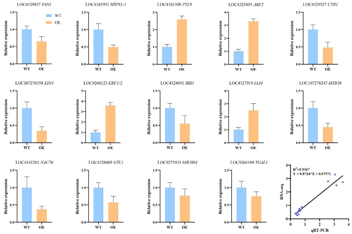
Supplementary Figure S4. qRT-PCR validation of DEGs in WT and HmWOX8 -OE. The bars represented standard deviation.
