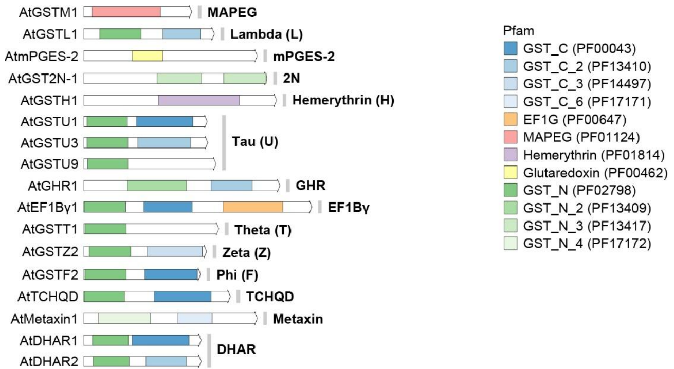
Fig. S1. Conserved domains of representative GST genes in Arabidopsis thaliana .
