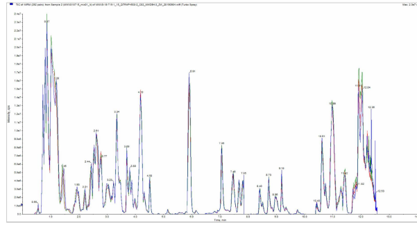
Supplementary Fig. 1 TIC of labellum of Cymbidium floribundum before and after pollination in different periods.
