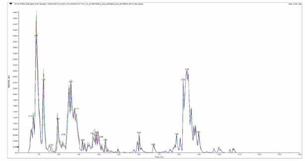
Supplementary Fig. 1 TIC of labellum of Cymbidium floribundum before and after pollination in different periods.
