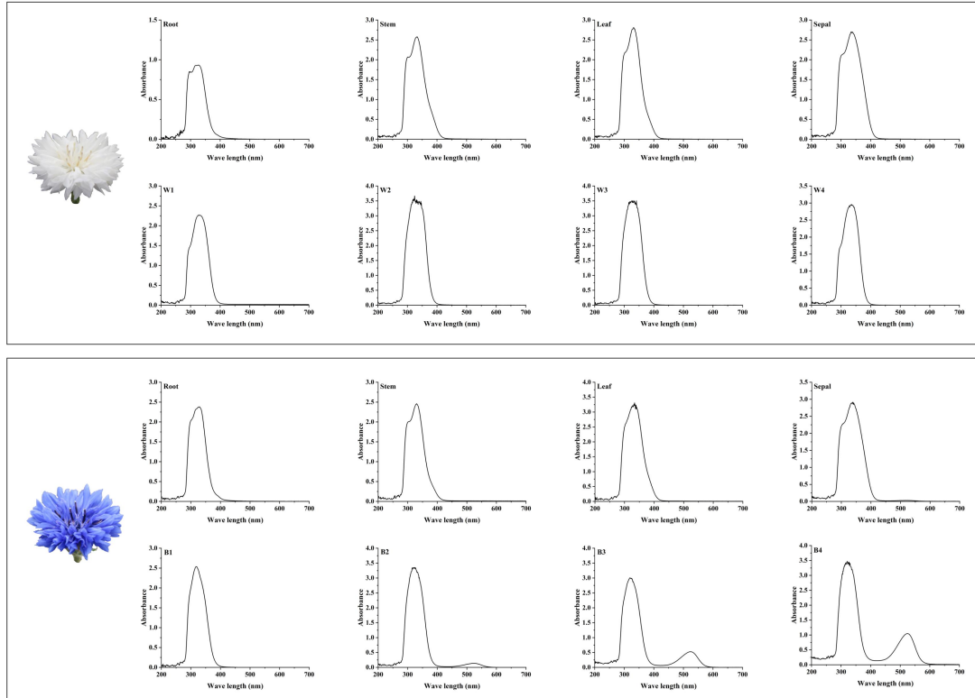
Fig. S1 The spectrum feature of extracts from different tissues of two cornflower cultivars detected by spectrophotometer.
