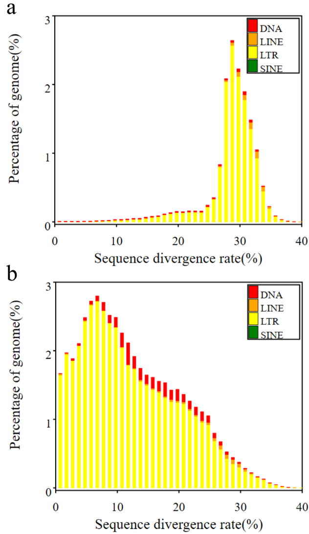
Figure S5. The sequence divergence rate of A. montana genome. a. The sequence divergence rate of four different TEs using RepeatMasker annotation. b. The sequence divergence rate of four different TEs using de novo annotation.
