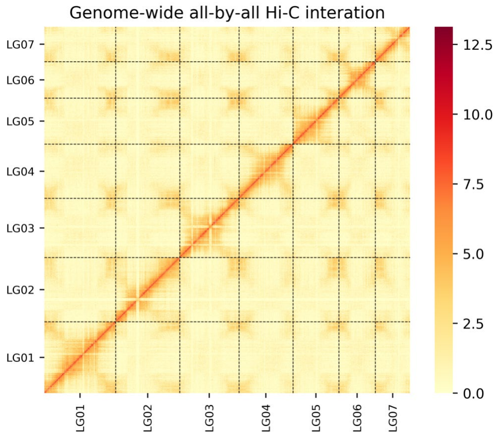
Figure S3. High-through chromosome conformation capture (Hi-C) contact data mapped to the genome of A. montana . The heat map represents the normalised contact matrix. The strongest contact is shown in red, the weakest contact is shown in yellow.
