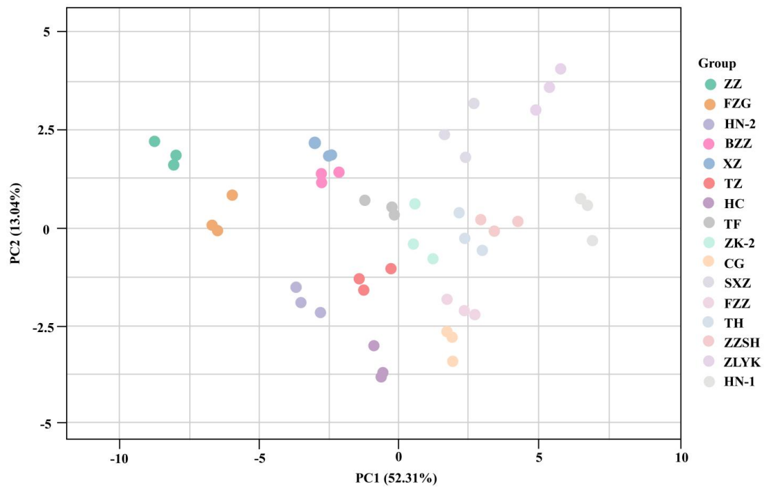
Supplemental Fig. S1. Principal component analysis with two factors.
