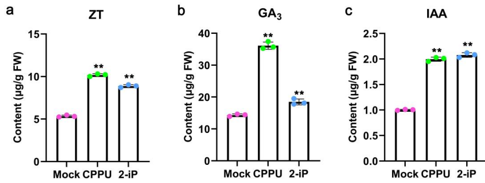
Figure S3. Endogenous ZT, GA 3 and IAA content in the control, CPPU and 2-iP treatment at BD16d during bulblet development in lily cultivar 'Matrix'. Data are represented as the means of three biological replicates with SD error bars (Student's t -test; **: p < 0.01).
