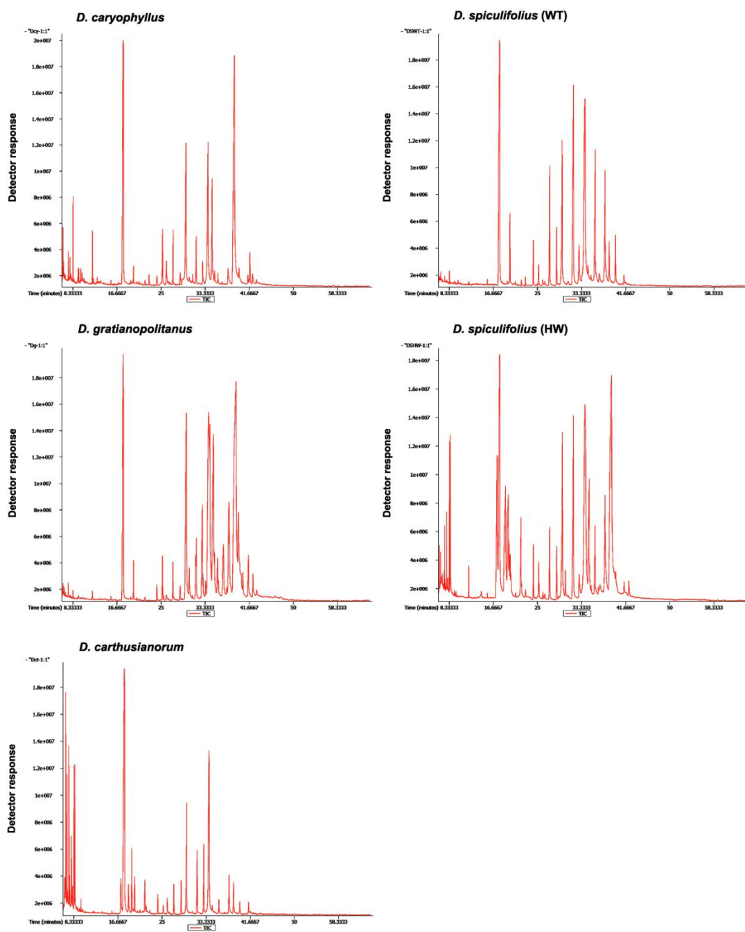
Fig. S2. Total ion chromatograms (TIC) of cuticular wax components extracted from the leaf surface of five Dianthus plants.
