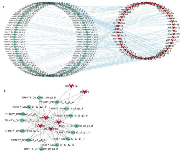
Supplementary Fig. S7. miRNA-target genes regulatory network. The green circle indicated the gene ID of the target genes, and the red arrow represented the miRNA. a: All miRNA-target genes regulatory network. b: miR156-SPLs regulatory network.
