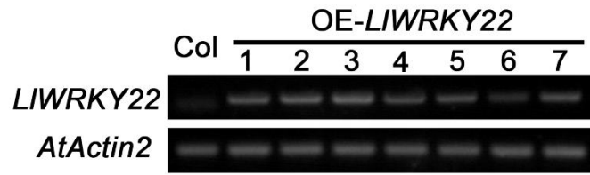
Fig. S1. Molecular analysis of LIWRKY22 transgenic Arabidopsis lines. The 5-day-old seedlings were used to detect the expression of LIWRKY22 in transgenic Arabidopsis lines by RT-PCR. PCR of the endogenous control and tested gene was performed with 28 and 30 cycles, respectively. AtActin2 was used as an endogenous control.
