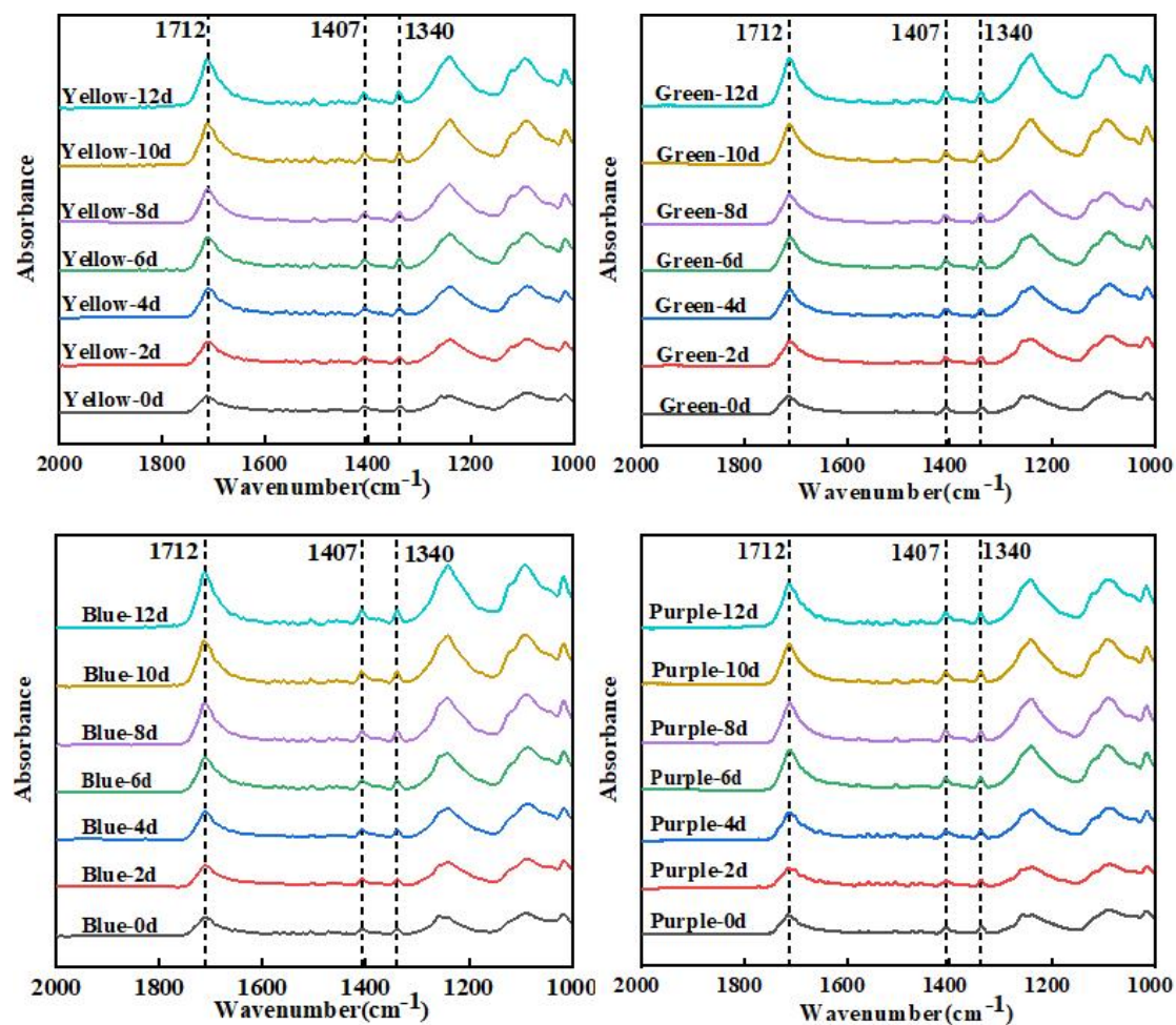
Supplementary Fig. S7 FTIR spectra of different colored PET sewing threads during UV exposure
