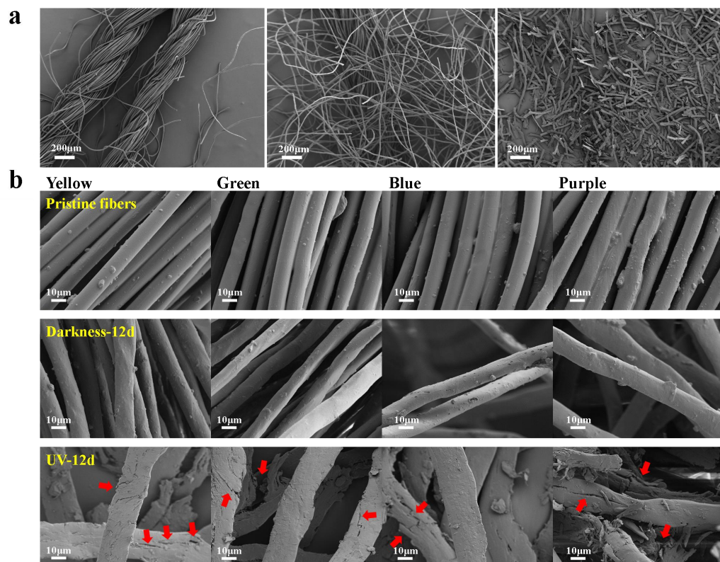
Supplementary Fig. S5 SEM of different colored PET fibers. (a) Fragmentation process of PET threads; (b) surface morphology changes of different PET fibers
