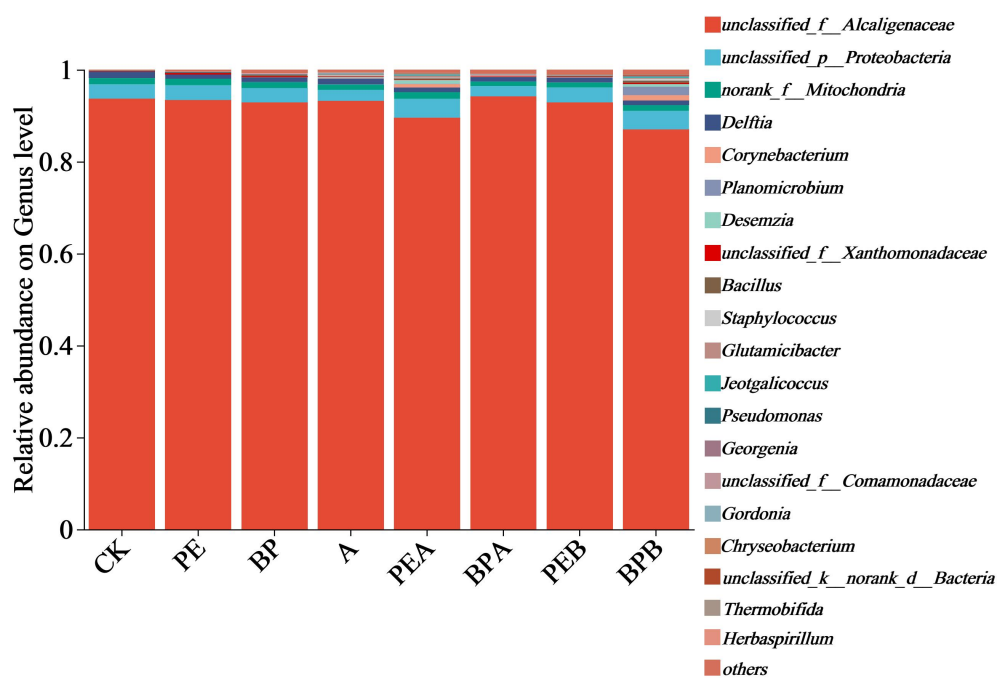
Figure S26 Bacterial communities at genus levels in soybean seed under different treatments.
