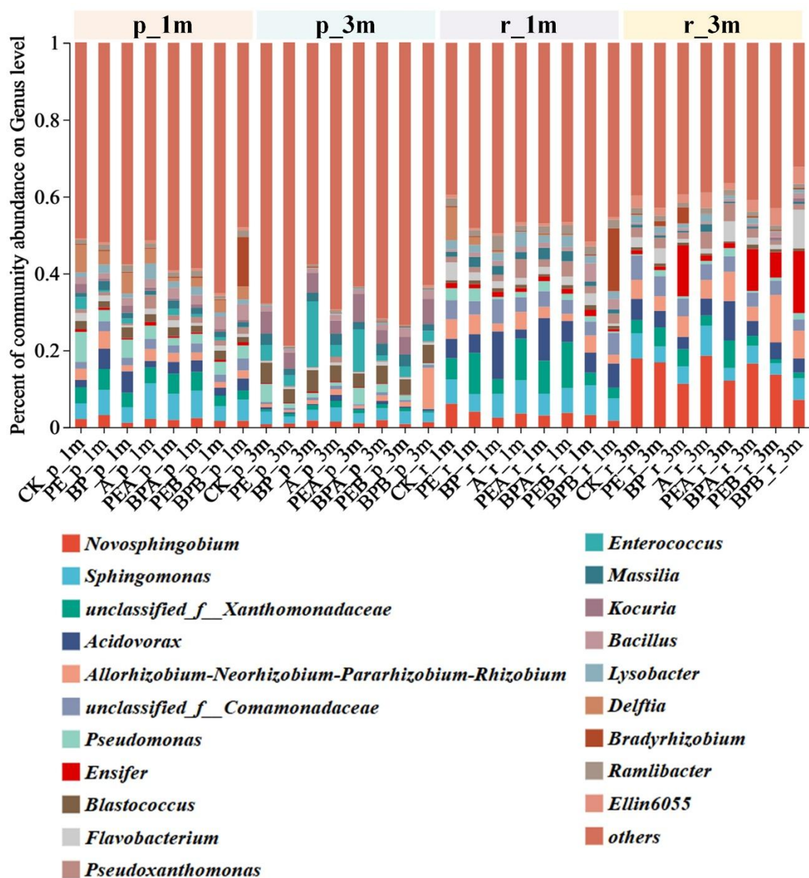
Figure S25 Bacterial communities at genus levels in soybean phyllosphere (p_1m and p_3m) and rhizoplane (r_1m and r_3m) under different treatments after incubation for 1 month and 3 months.
