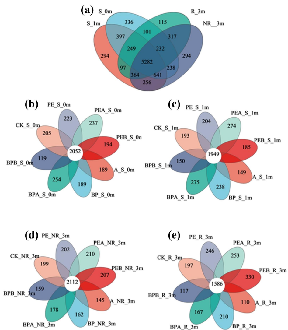
Figure S18 Venn diagram showing the number of unique and shared operational taxonomic units (OTUs) of soil bacteria between different treatments.
