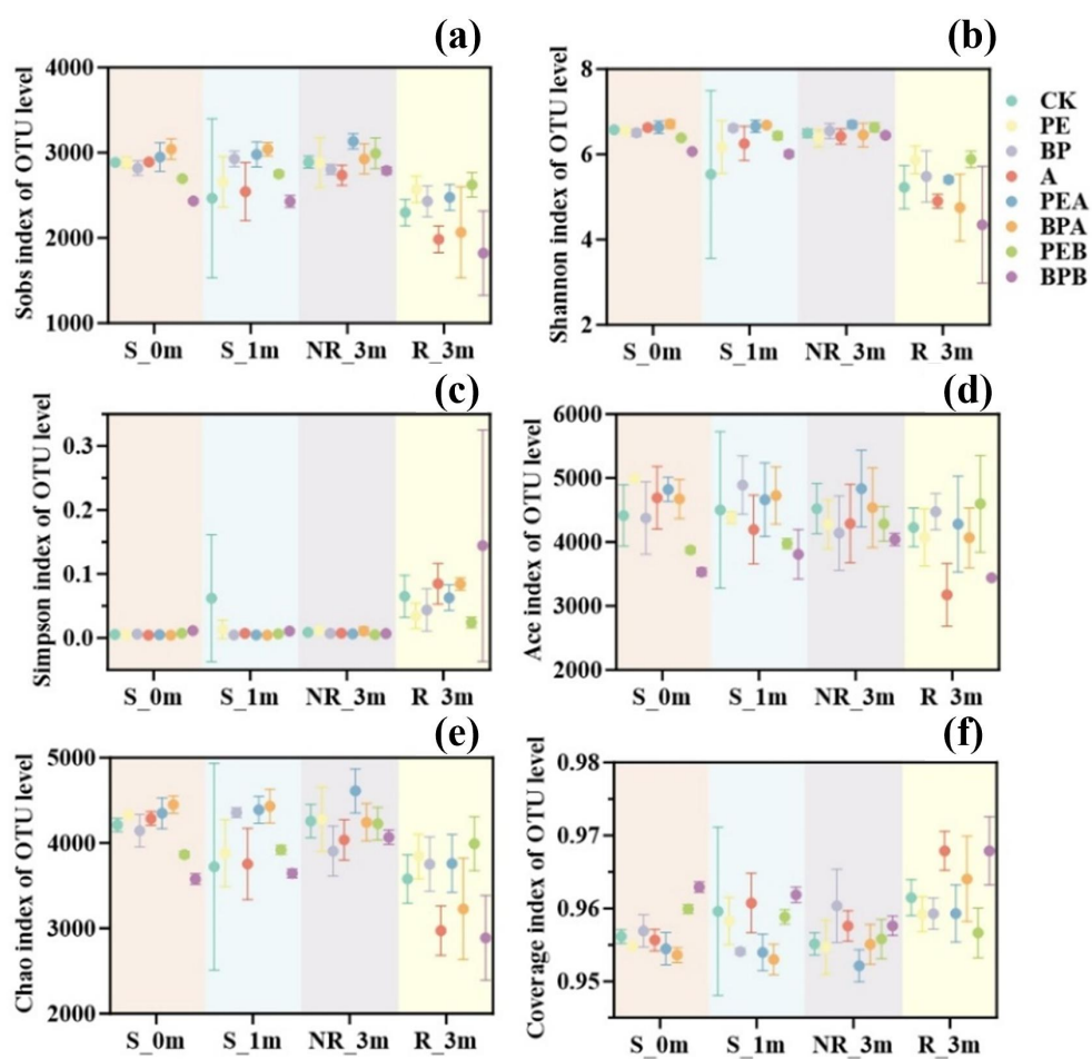
Figure S13 Variations in bacterial alpha diversity under different treatments in soil samples.
