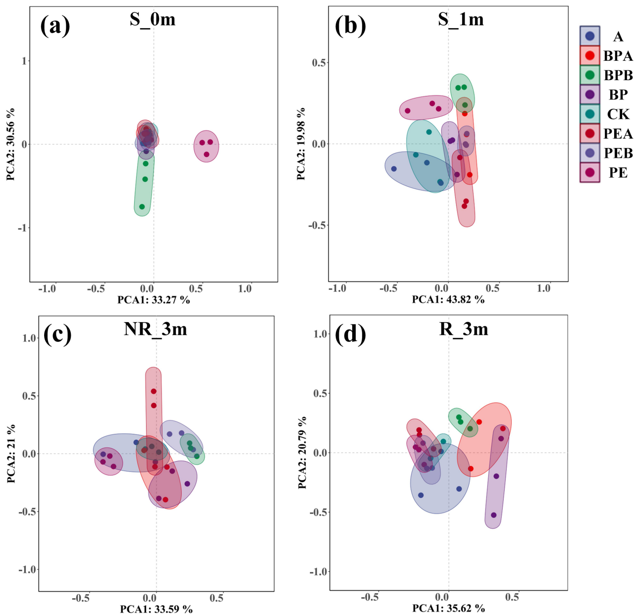
Figure S10 Principal component analysis (PCA) shows the overall distribution pattern of ARGs in the different treatments at the beginning of the experiment soil (S_0m), after incubation for 1 month soil (S_1m), after incubation for 3 months non-rhizosphere soil (NR_3m) and rhizosphere soil (R_3m).
