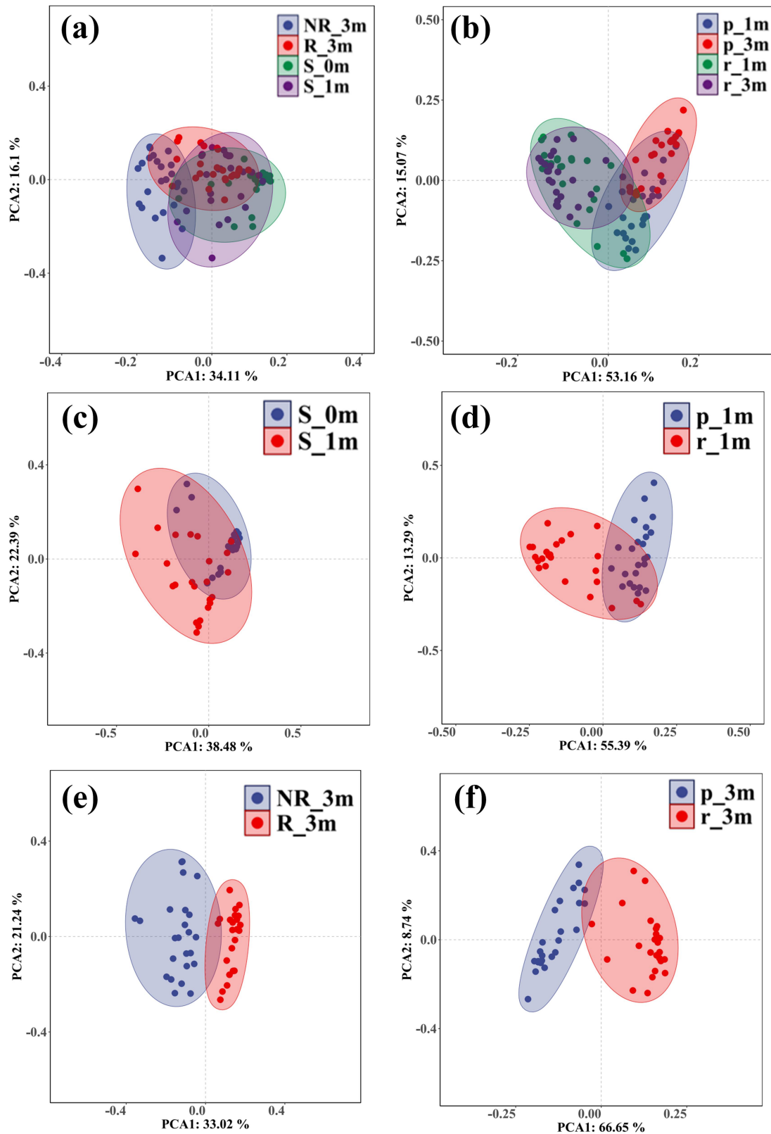
Figure S9 Principal component analysis (PCA) shows the overall distribution pattern of ARGs in different habitats and different growth periods.
