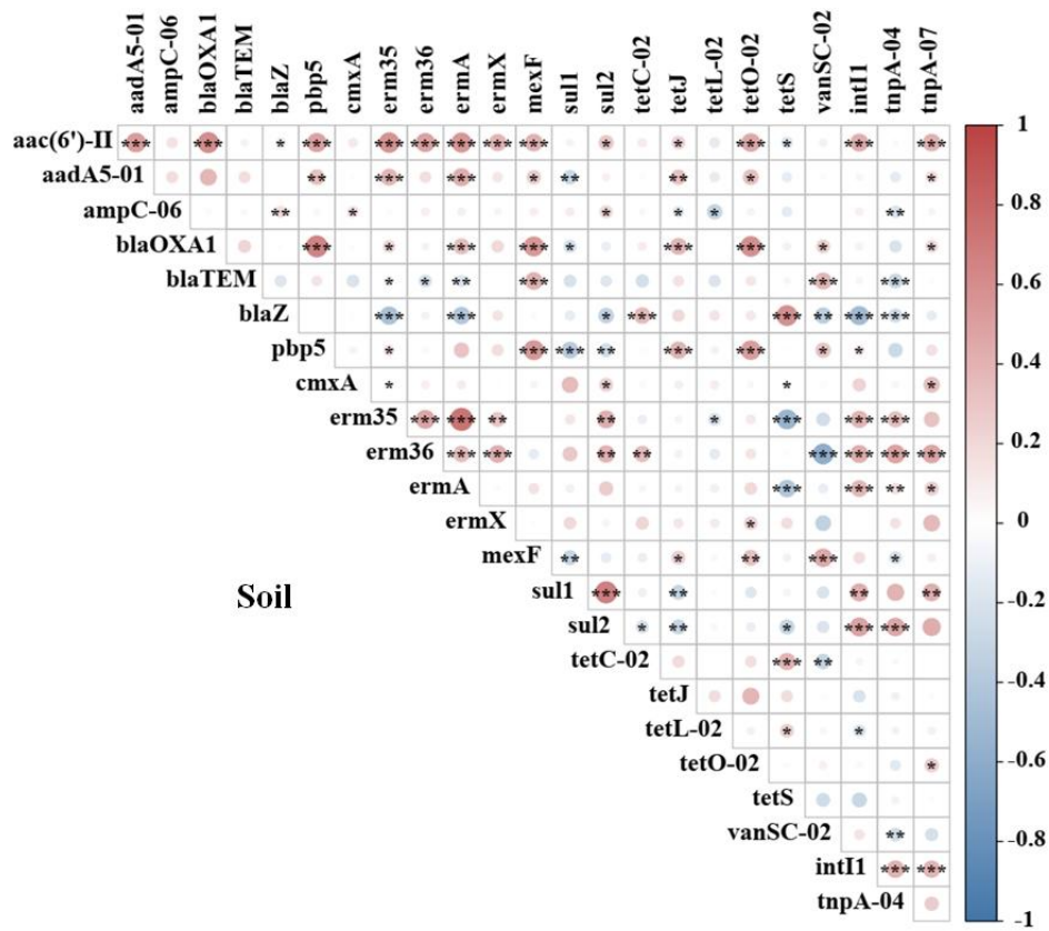
Figure S7 Heatmap shows the correlation between the ARGs and MGEs in soil. * 0.01 < p \leq 0.05 , ** 0.001 < p \leq 0.01 , *** p \leq 0.001 .
