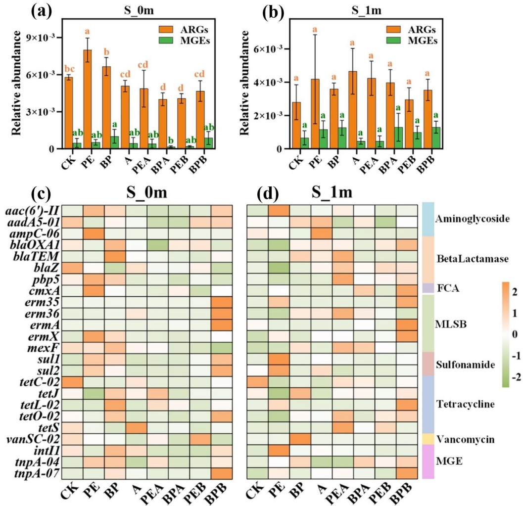
Figure S4 Relative abundance of antibiotic resistance genes (ARGs) and mobile genetic elements (MGEs) at (A and C) the beginning of the experiment (S_0m) and (B and D) after incubation for 1 month (S_1m) under different treatments. Error bars represent standard deviations (n=3). Lowercase letters indicate significant differences between treatments.
