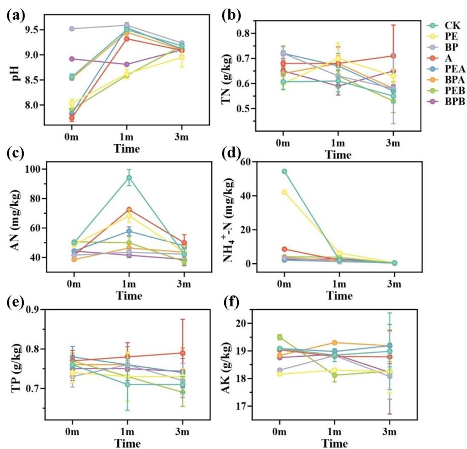
Figure S3 Soil physical-chemical properties under different treatments at the beginning of the experiment (0m), and after incubation for 1 month (1m) and 3 months (3m).
