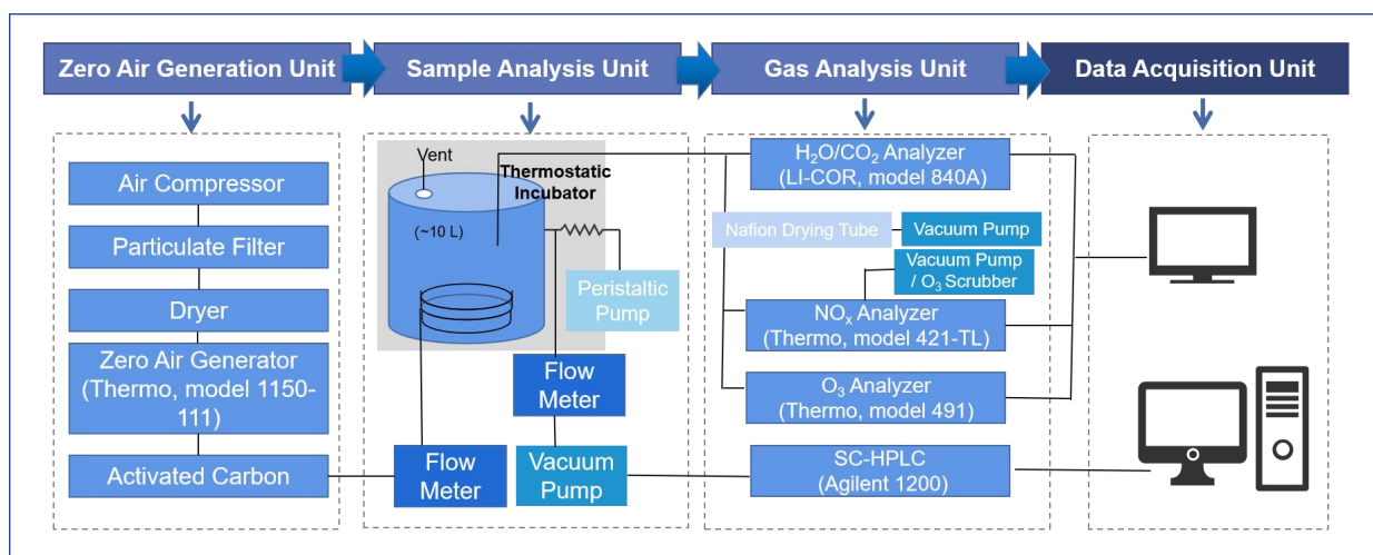
Fig. S2 The schematic diagram of the dynamic chamber measurement system. The diagram was adapted from Deng [1] .
