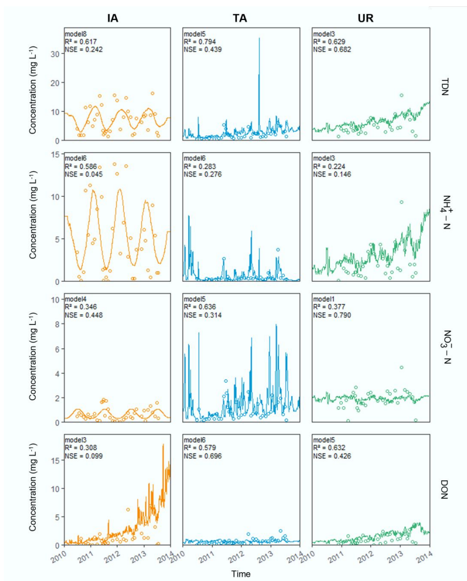
Fig. S2 Daily simulated concentrations of nitrogen species across the three study watersheds generated using LOADEST models.
