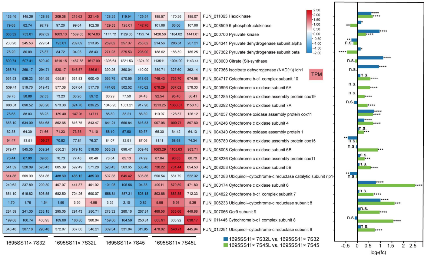
Figure S14. Transcriptional changes of key enzymes involved in glycolysis and the tricarboxylic acid (TCA) cycle. Significance was assessed using DESeq2 (n.s., not significant; *, q < 0.05 , **, q < 0.01 , ***, q < 0.001 , ****, q < 0.0001 ).
