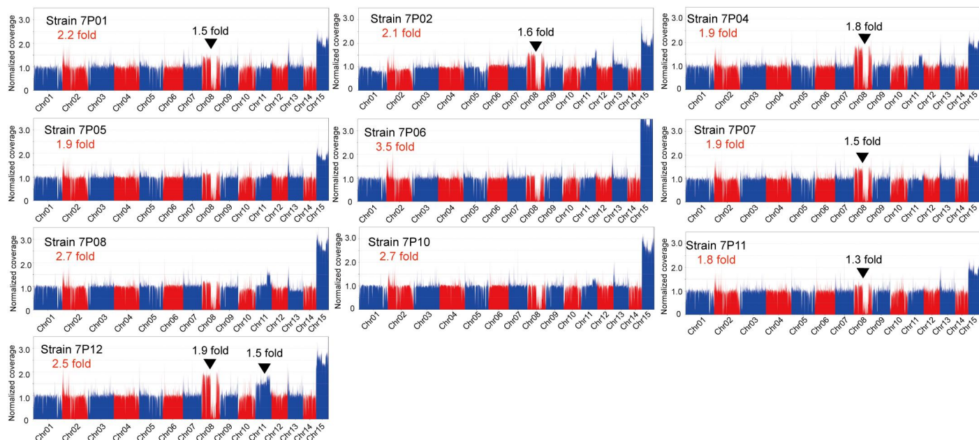
Figure S24. CC aneuploidy events in ten protoplast-regenerated strains derived from strain 776. Strain IDs (black) and copy number of AC (red) inferred from normalized coverage were shown at the top. Triangles indicate CC aneuploidy events.
